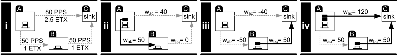
Figure 2: A three node network is given in (i), links are labeled with both rate and expected transmission count per packet. Bold links in (ii) through (iv) indicate links selected for packet forwarding. Weights are calculated using Equation (5) with V = 1 .
