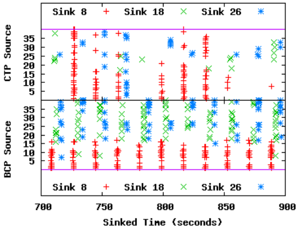
Figure 12: Results from highly mobile sink experiments, we present a 200 second window of sink time versus source mote for sinks 8, 18 and 26 running CTP (top) and BCP (bottom). Each Sink in BCP services communities of nodes having low ETX, while CTP attempts to rebuild trees that service the entire network.
