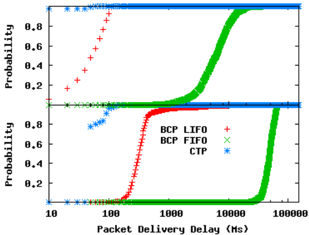
Figure 5: Source to sink delay CDF at 0.25 PPS for notes 4 and 40 under CTP, BCP-FIFO and BCP-LIFO.
