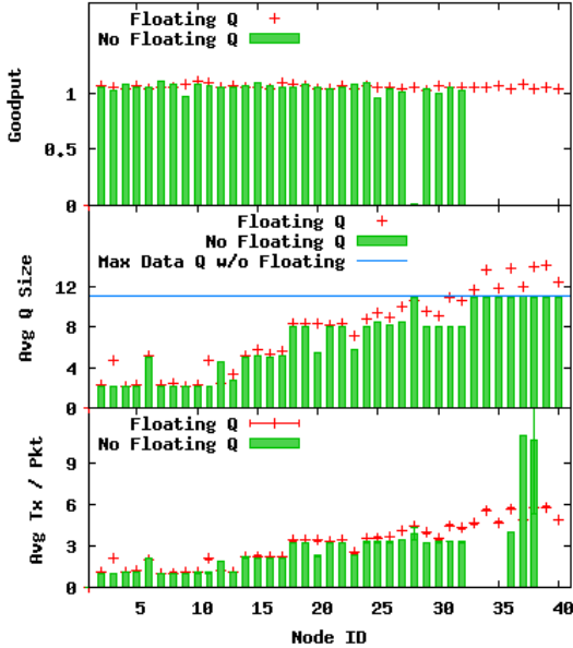
Figure 7: Comparison of BCP’s per mote goodput, time average queue sizes and average packet transmissions for sinked packets with 95% confidence intervals. Tests are run with and without BCP’s floating queues disabled. The maximum data queue size is 11.
