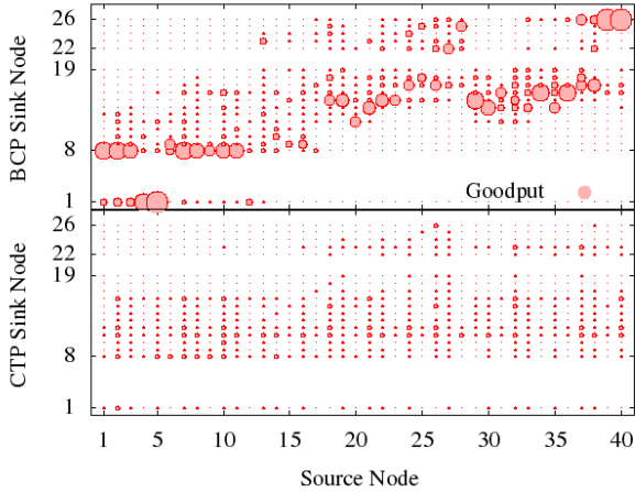
Figure 11: Results from highly mobile sink experiments on BCP (top) and CTP (bottom). Circle radius represents the goodput received by the sink (row) originated by the source (column). Gradients in BCP direct packets to the most efficient regional sinks.
