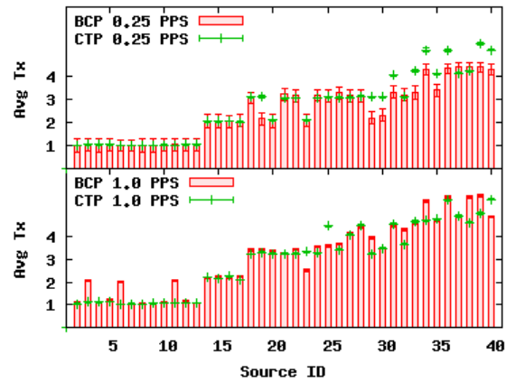
Figure 9: Per source average per packet transmission count to the sink and 95% confidence intervals for static tests at 0.25 PPS (top) and 1.0 PPS (bottom) on CTP and BCP.
