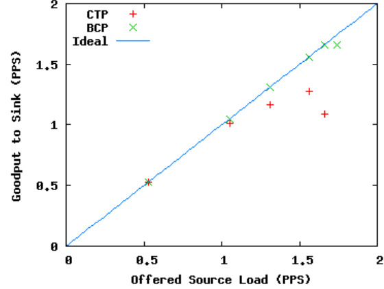
Figure 8: Goodput in static tests over source rate for CTP, BCP and Volcano.
